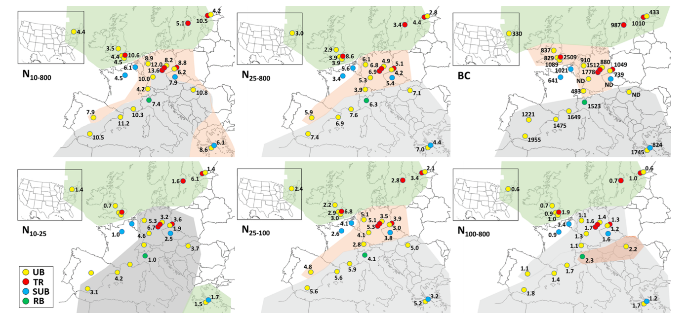
Fig. 3. Regional variability of averaged 2017–2019 particle number concentrations (in \# \text{cm}^{-3} 10^{-3} ) size fractions (in \# \text{cm}^{-3} 10^{-3} ) and black carbon (BC in \text{ng m}^{-3} ) in Europe. For N_{10-25} , only sites with a lower size detection limit of 10–14 nm are included. UB, Urban background; TR, traffic; SUB, Suburban background; RB, Regional background. Shaded areas include the UB sites recording the lowest (green), intermediate (orange) and highest (grey) concentrations. (For interpretation of the references to colour in this figure legend, the reader is referred to the web version of this article.)
